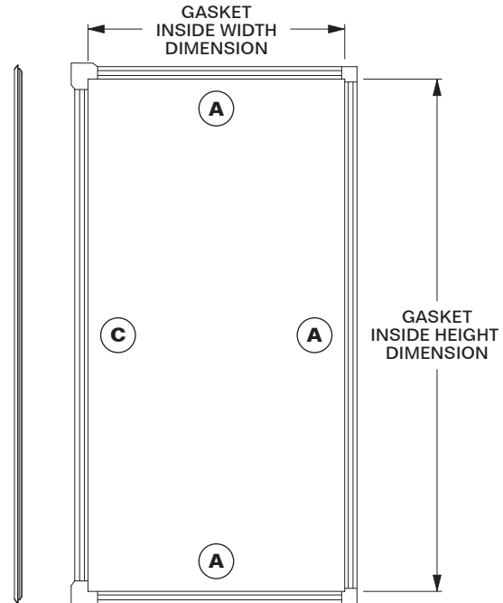
MODEL 1404-8954-R (8'6") MODEL 1404-8955-R (9'6") DOOR GASKET, Combo Design Inner & Outer, Right
